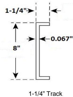
Figure 4 – Track/Ledger
