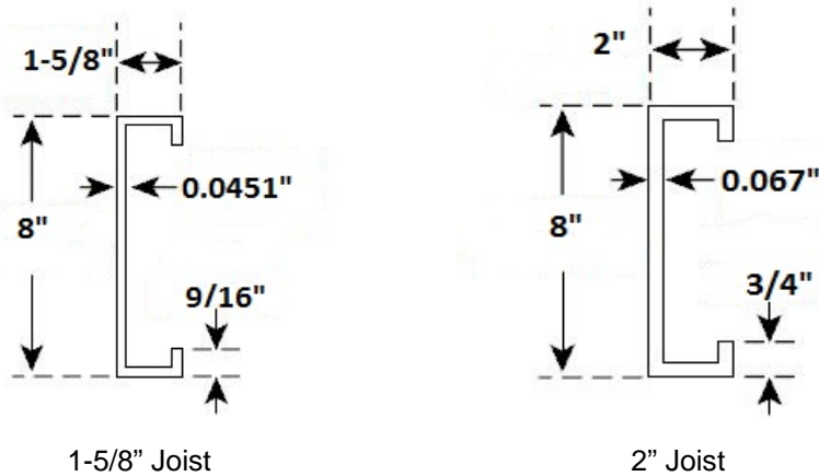
Figure 3 – Steel Joists
